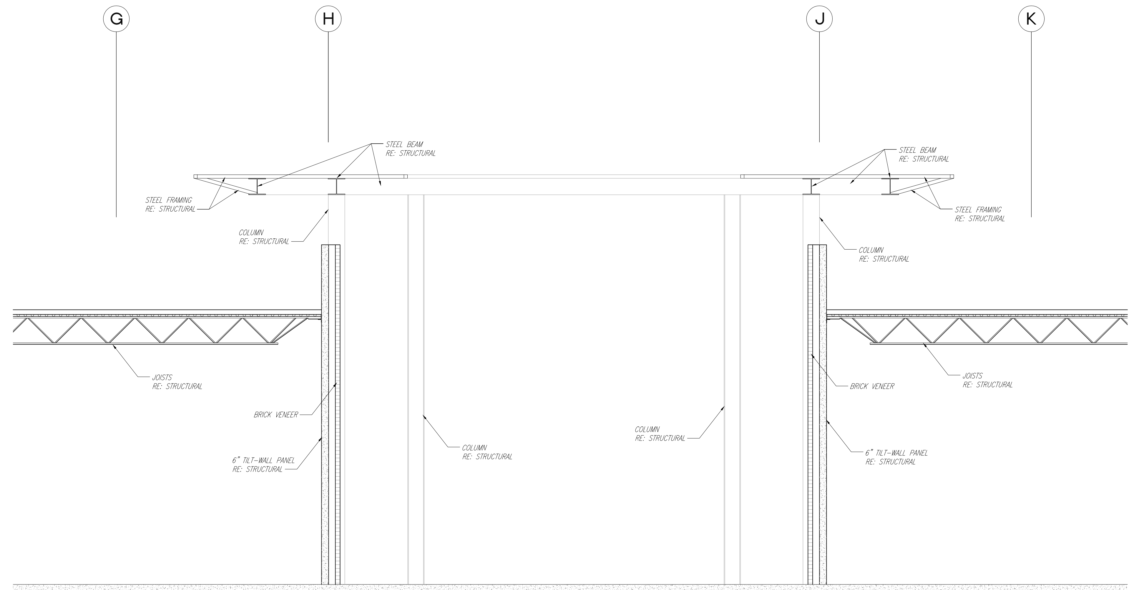
2 CANOPY SECTION SCALE: 1/4" = 1'-0"
